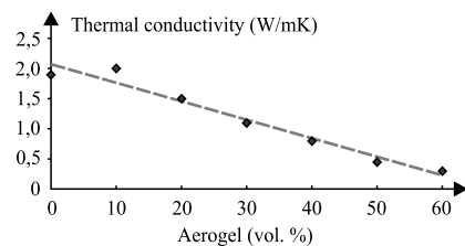
Fig. 1. Aerogel volume content vs. thermal conductivity in mortars
